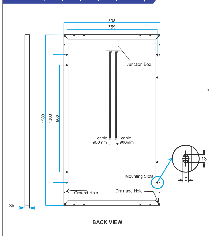
MCA-200, 205, 210, 215, 220, 225 Wp
